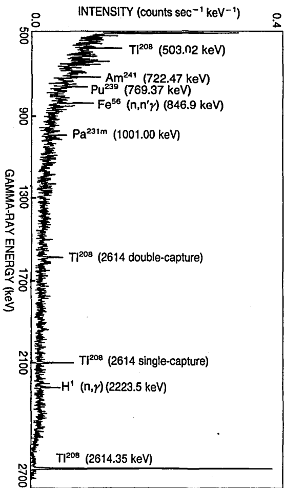
Figure 1: The gamma-ray signal recorded by a germanium detector placed on top of a cruise-missile launcher 3.4 meters from the lid for 10 minutes
